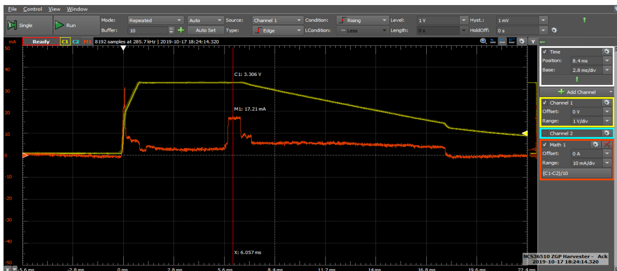
Figure 5: Waveforms of Regulated Supply (Yellow) and Device Current Consumption (Red)
