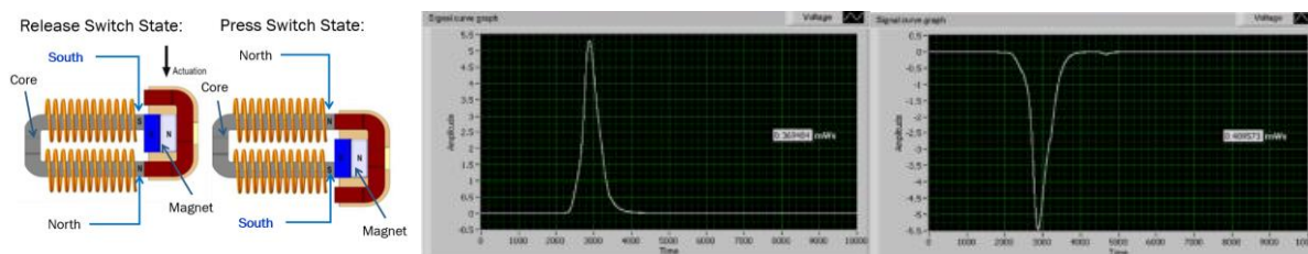
Figure 4: Energy Harvesting Power Generation
