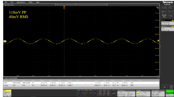
Figure 30 - VBUSOUT ripple for 15V/0A
