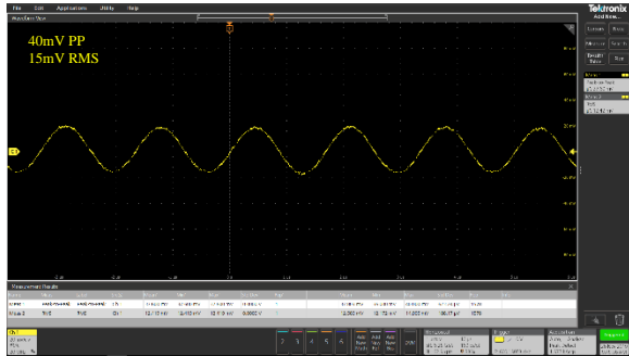
Figure 23 - VBUSOUT ripple for 5V/3A
