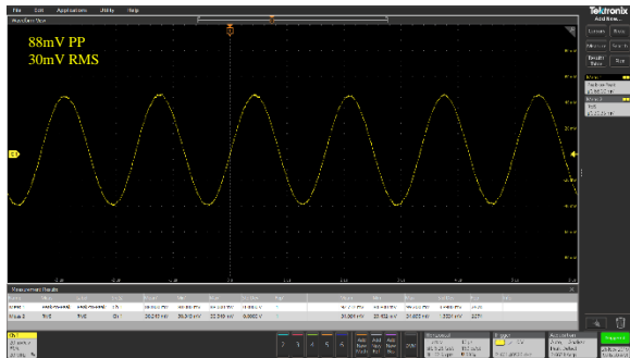
Figure 25 - VBUSOUT ripple for 9V/3A
