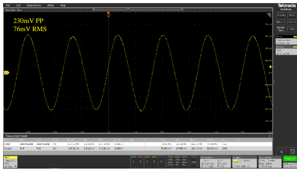
Figure 31 - VBUSOUT ripple for 20V/3A
