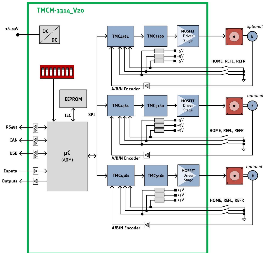
Figure 10.1 Main parts of the TCM314
