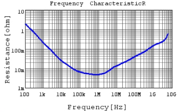
GRM155R60J106ME15 R DCOV, 25degC
