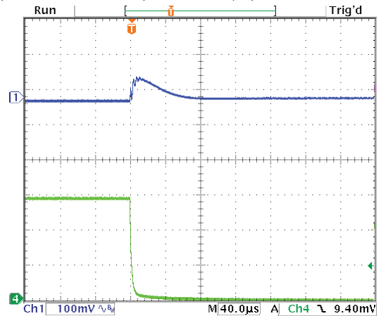
Step Load Transient Response (Vin=12V, Vout=1.8V, Cload=10x10µF X5R 0805 ceramic, plus 1x470µF, 7mΩ POSCAP, total 570µF, Iout=3A to 0A) Top trace=Vout, Bottom trace=Iout
