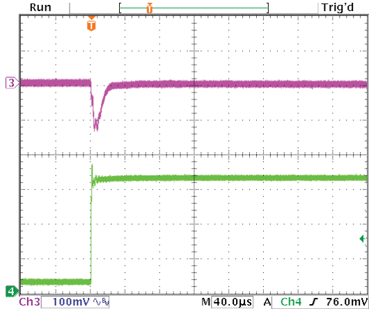
Step Load Transient Response (Vin=7.5V, Vout=5V, Cload=5x10µF X5R 0805 ceramic, total 50µF, Iout=0A to 3A) Top trace=Vout, Bottom trace=Iout
