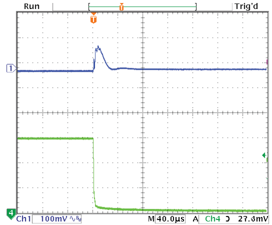
Step Load Transient Response (Vin=4.5V, Vout=1.8V, Cload=10x10µF X5R 0805 ceramic, plus 1x470µF, 7mΩ POSCAP, total 570µF, Iout=3A to 0A) Top trace=Vout, Bottom trace=Iout
