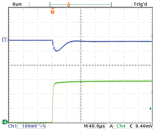
Step Load Transient Response (Vin=12V, Vout=1.8V, Cload=10x10µF X5R 0805 ceramic, plus 1x470µF, 7mΩ POSCAP, total 570µF, Iout=0A to 3A) Top trace=Vout, Bottom trace=Iout
