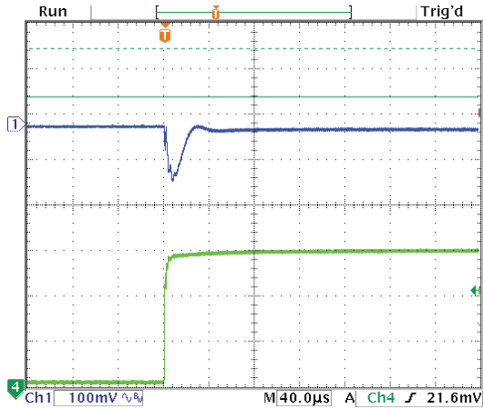
Step Load Transient Response (Vin=4.5V, Vout=1.8V, Cload=10x10µF X5R 0805 ceramic, plus 1x470µF, 7mΩ POSCAP, total 570µF, Iout=0A to 3A) Top trace=Vout, Bottom trace=Iout
