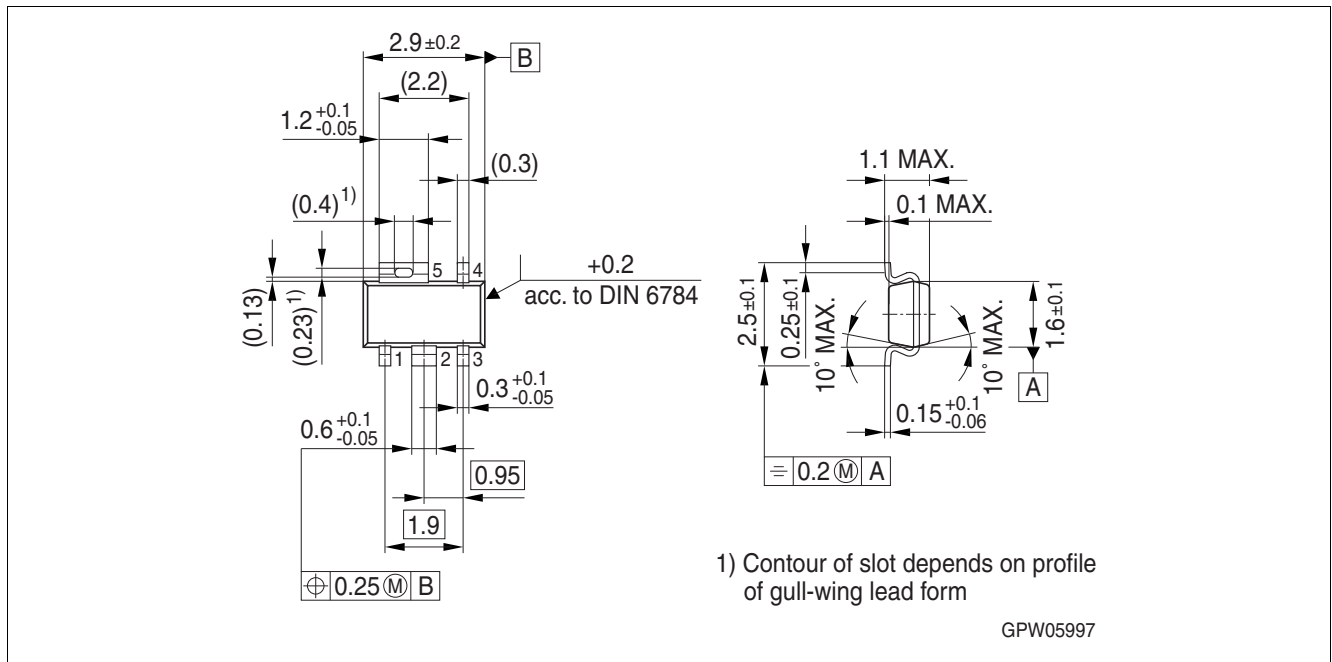
Figure 3 Outline PG-SCT595-5 ¹)
