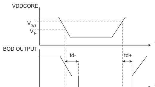
Figure 57-1. Core Brownout Output Waveform
