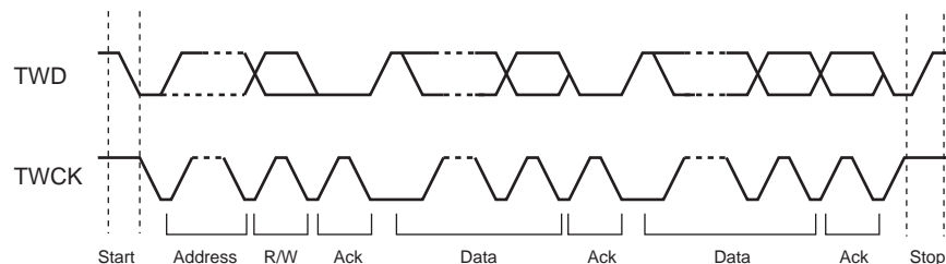
Figure 42-3. Transfer Format
