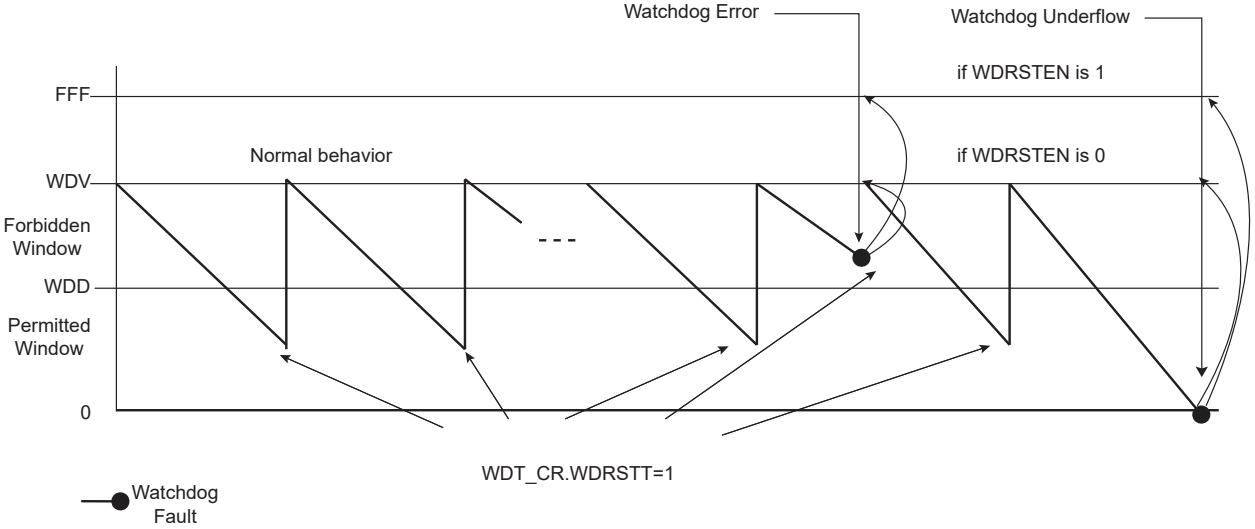
Figure 24-2. Watchdog Behavior
