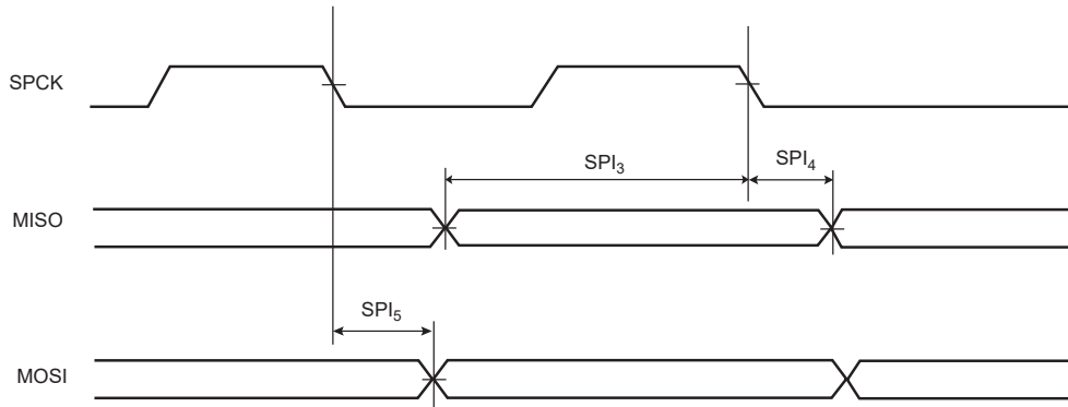
Figure 58-22. SPI Client Mode with (CPOL=0 and NCPHA=1) or (CPOL=1 and NCPHA=0)
