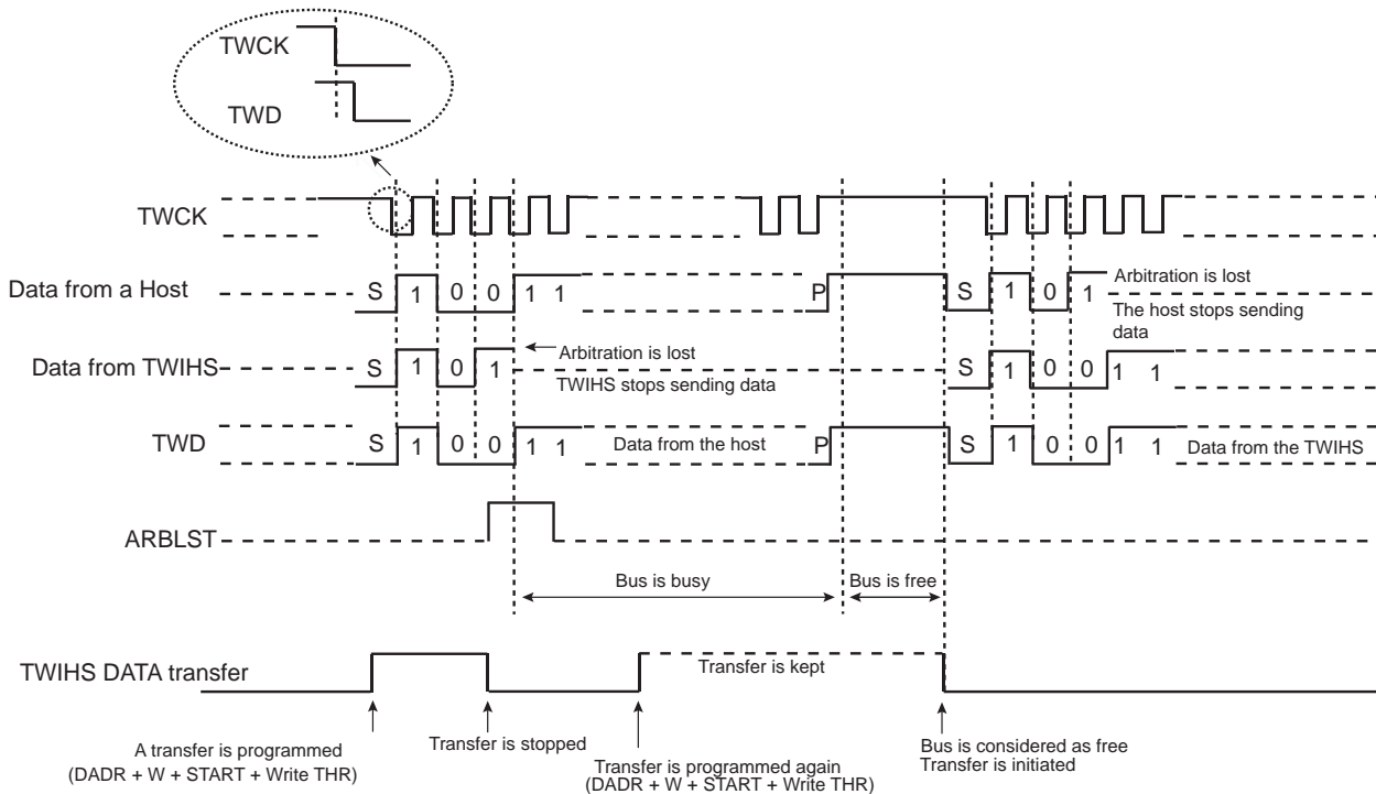
Figure 42-29. Arbitration Cases
