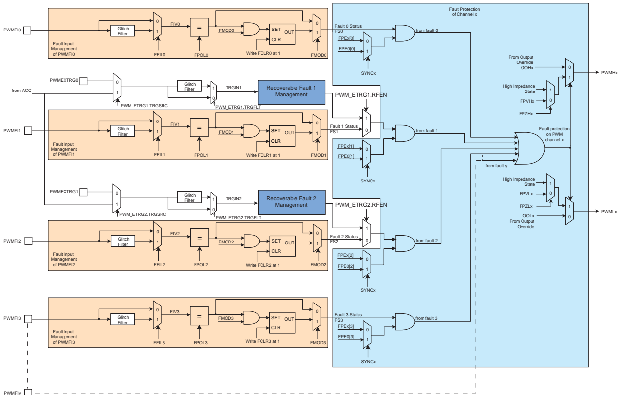
Figure 50-16. Fault Protection
