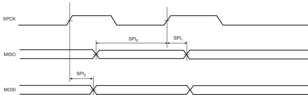
Figure 58-20. SPI Host Mode with (CPOL= NCPHA = 0) or (CPOL= NCPHA= 1)
