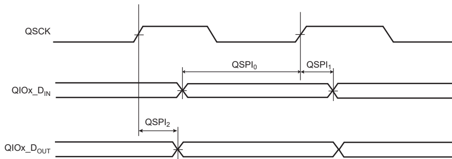
Figure 57-18. QSPI Host Mode with (CPOL = CPHA = 0) or (CPOL = CPHA = 1)
