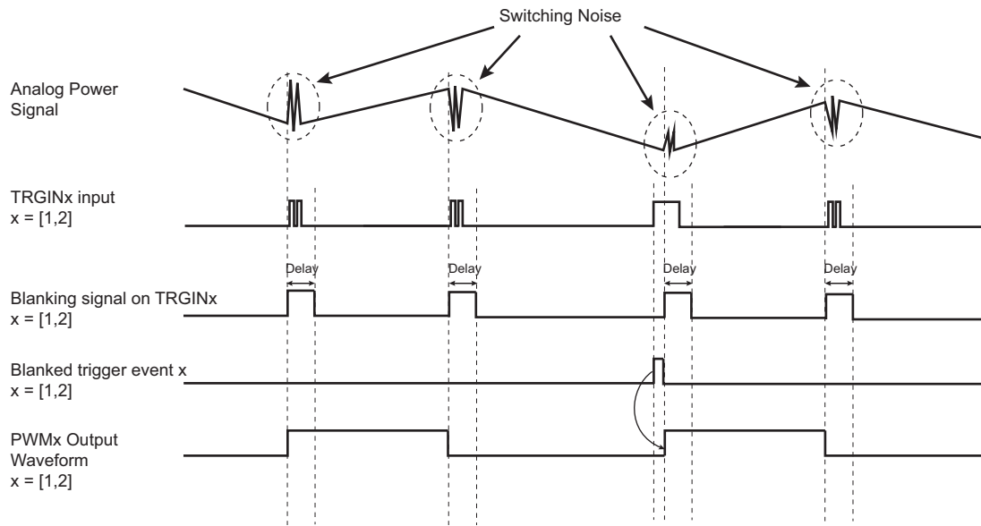
Figure 50-33. Leading-Edge Blanking
