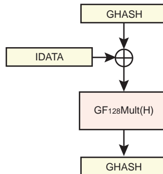
Figure 56-7. Single \text{GHASH}_H Block Diagram (AADLEN \leq 0x10 and CLEN = 0)
