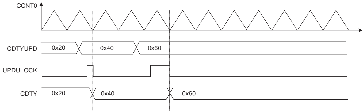
Figure 50-19. Method 1 (UPDM = 0)
