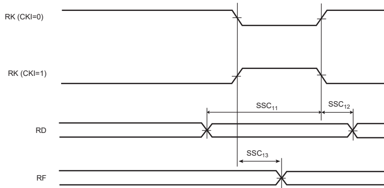
Figure 58-38. SSC Receiver, RK in Output and RF in Input
