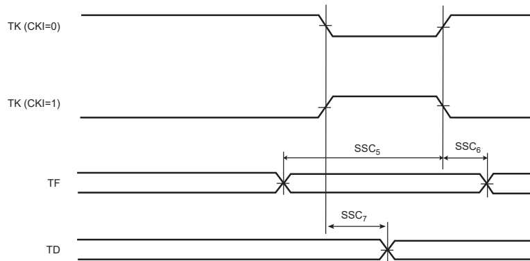
Figure 58-35. SSC Receiver RK and RF in Input
