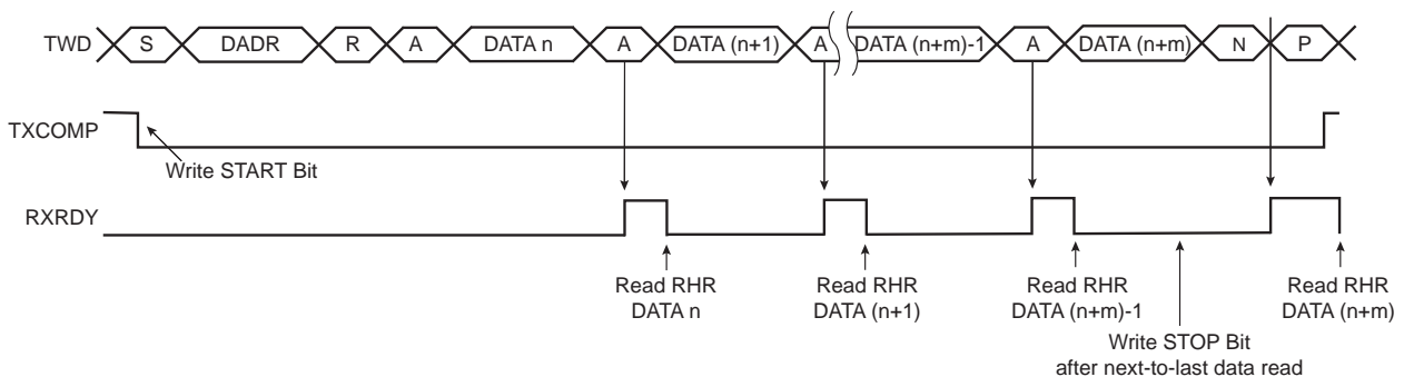
Figure 42-8. Host Read with Multiple Data Bytes
