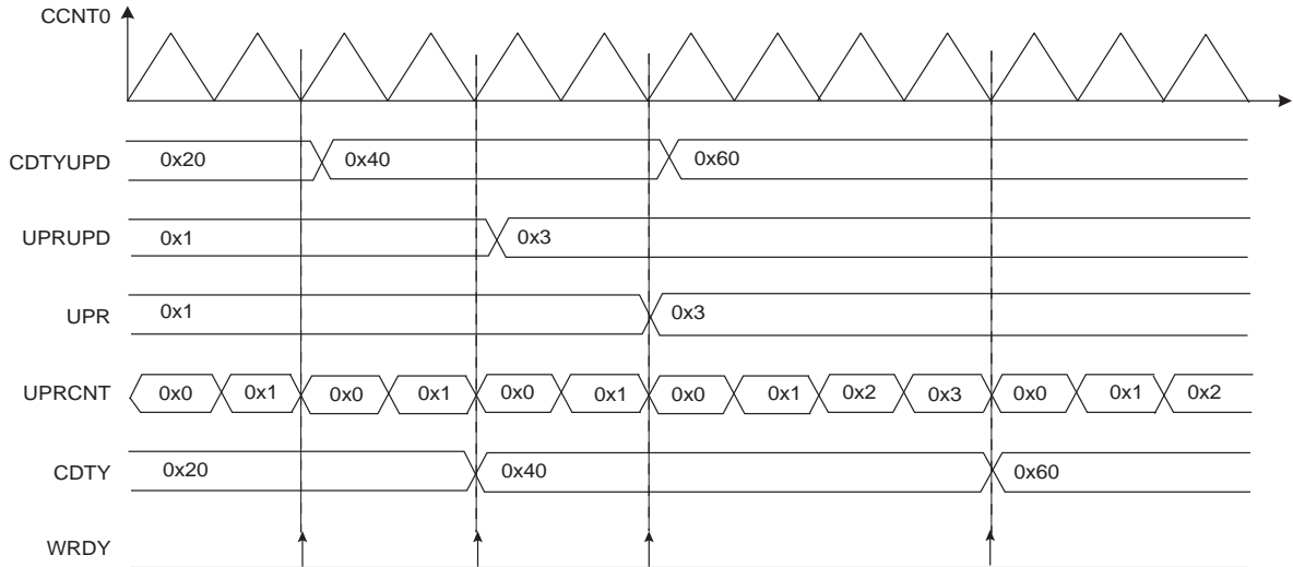
Figure 50-20. Method 2 (UPDM = 1)
