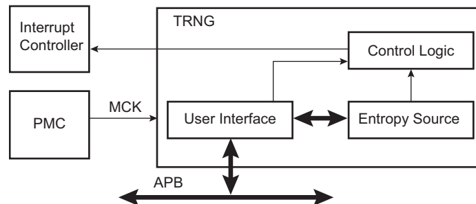
Figure 55-1. TRNG Block Diagram
