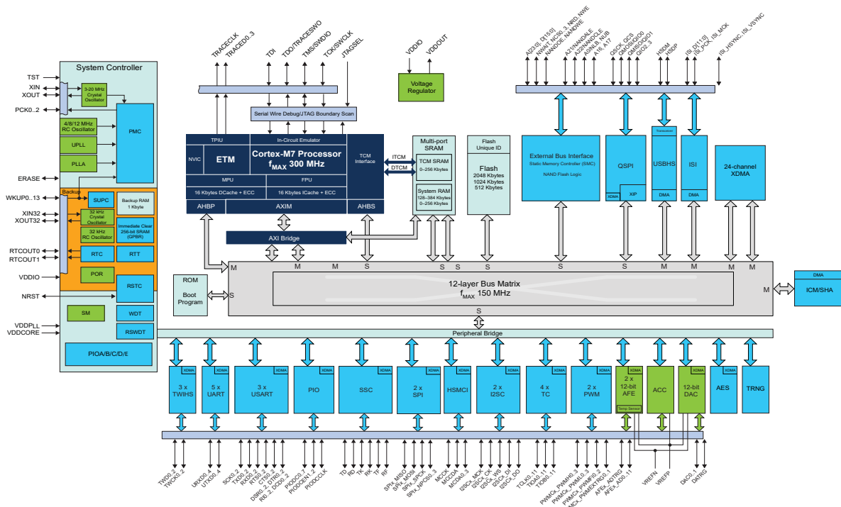
Figure 3-1. SAM S70 144-pin Block Diagram
