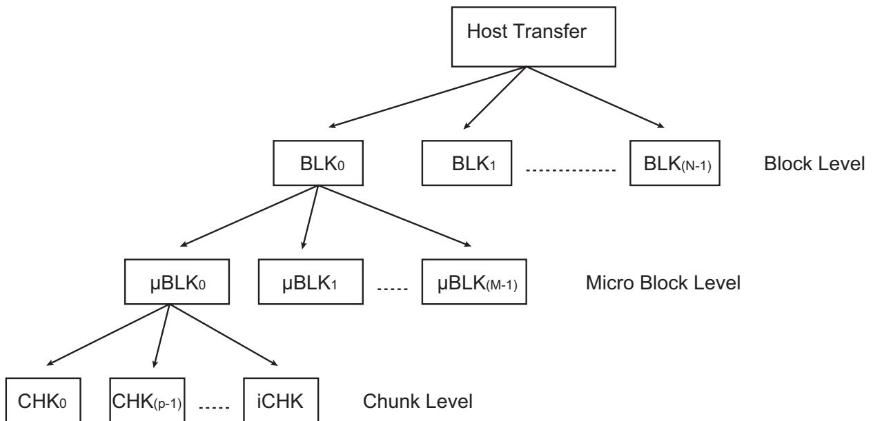
Figure 35-3. XDMAC Peripheral Transfer Hierarchy
