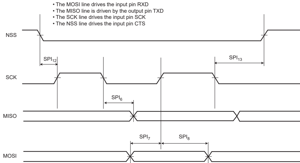
Figure 58-26. USART SPI Client Mode (Mode 0 or 3)
