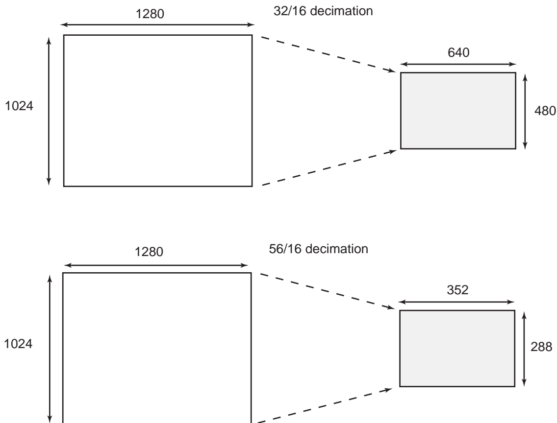
Figure 36-5. Resize Examples
