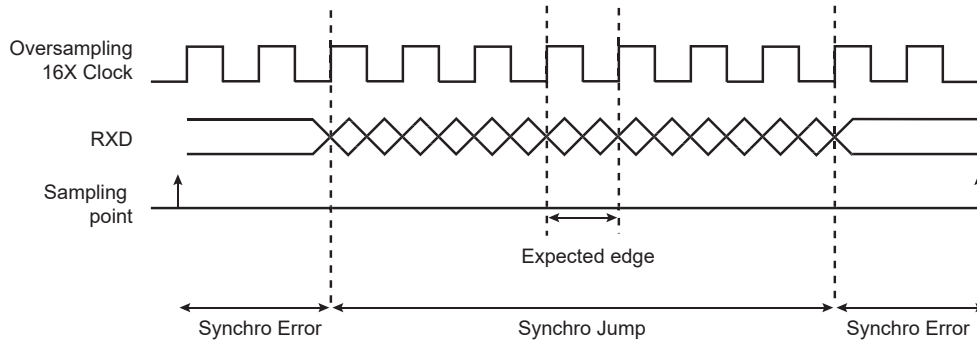
Figure 45-60. Bit Resynchronization
