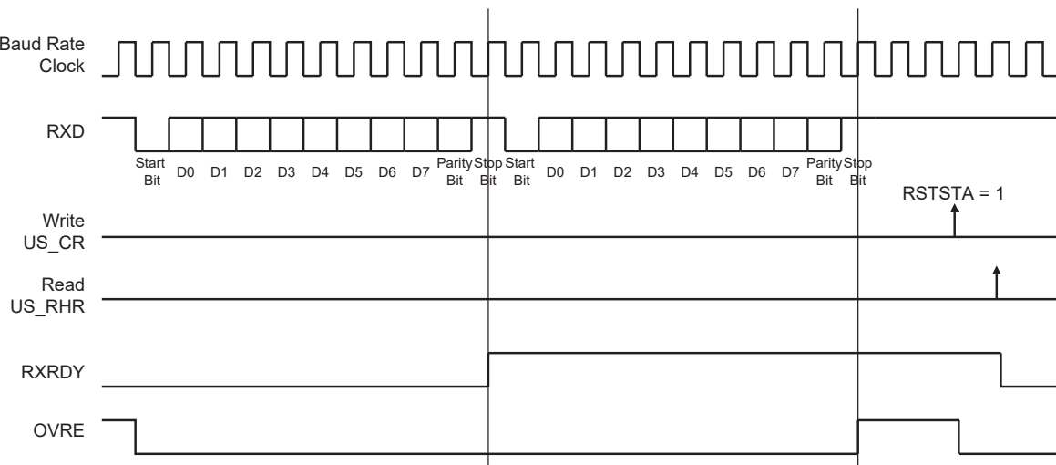
Figure 45-20. Receiver Status
