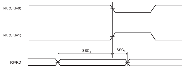
Figure 58-36. SSC Receiver, RK in Input and RF in Output
