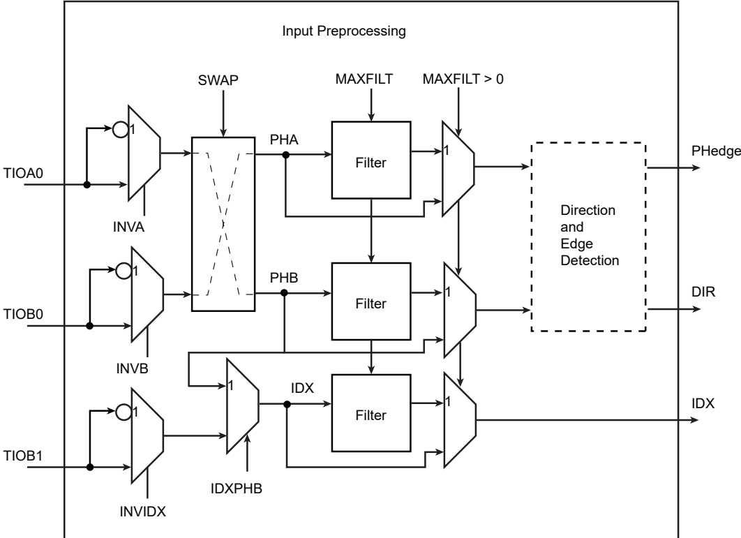
Figure 49-18. Input Stage
