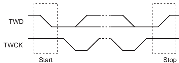
Figure 42-2. START and STOP Conditions
