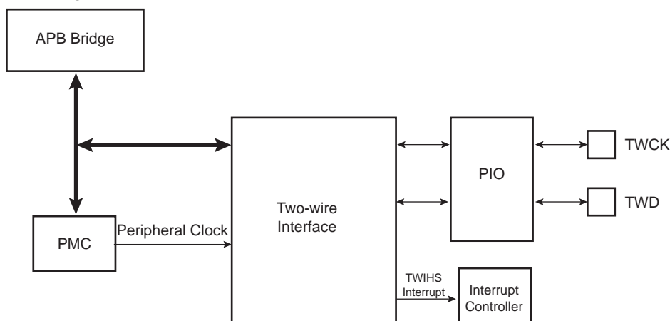
Figure 42-1. Block Diagram
