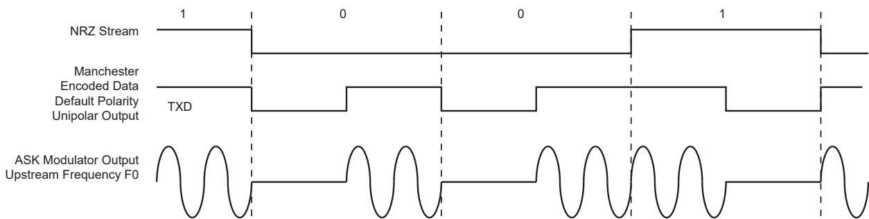
Figure 45-17. ASK Modulator Output
