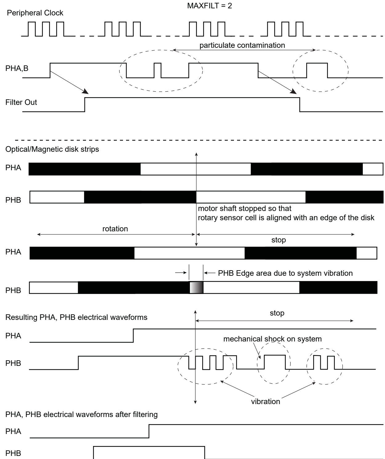
Figure 49-19. Filtering Examples
