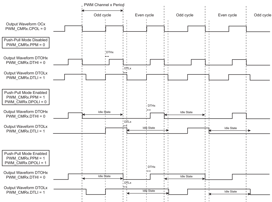
Figure 50-10. PWM Push-Pull Mode
