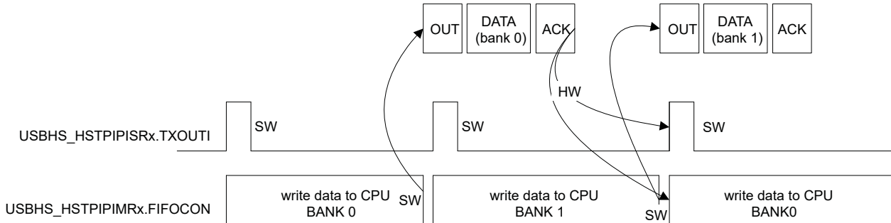
Figure 38-23. Example of an OUT Pipe with two Data Banks and a Bank Switching Delay
