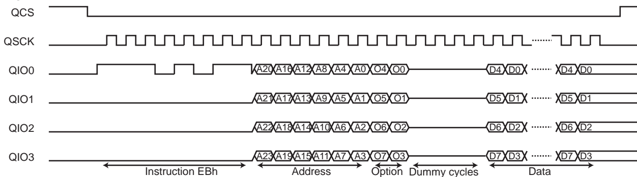
Figure 41-8. Instruction Frame
