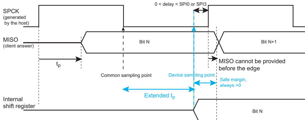
Figure 58-20. SPI Host Mode with (CPOL= NCPHA = 0) or (CPOL= NCPHA= 1)
