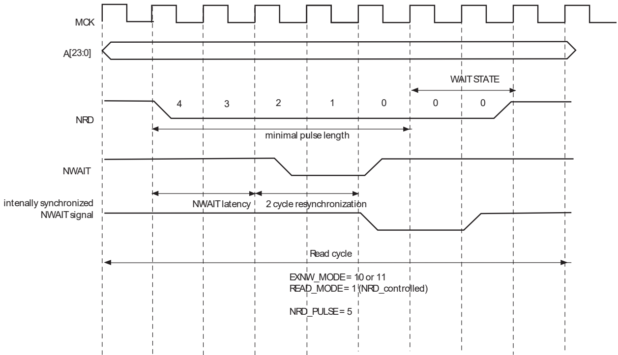
Figure 34-31. NWAIT Latency
