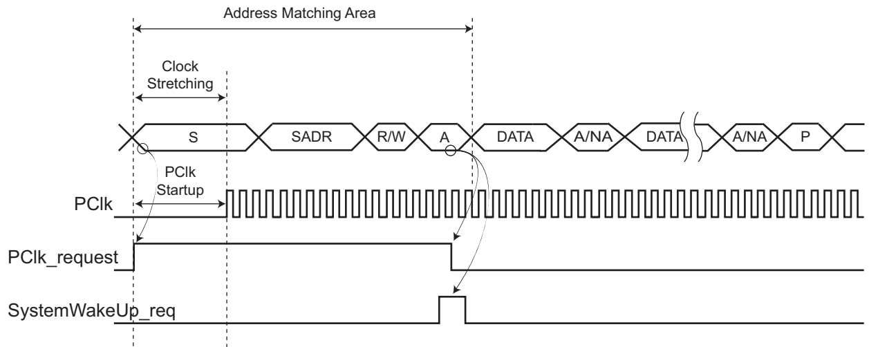
Figure 42-40. No Address Match (Data Matching Disabled)
