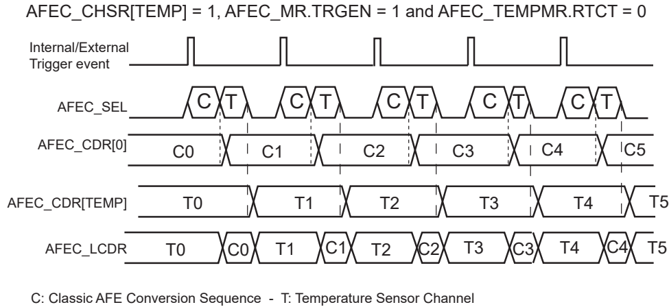
Figure 51-8. Non-Optimized Temperature Conversion
