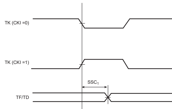
Figure 58-32. SSC Transmitter, TK in Input and TF in Output
