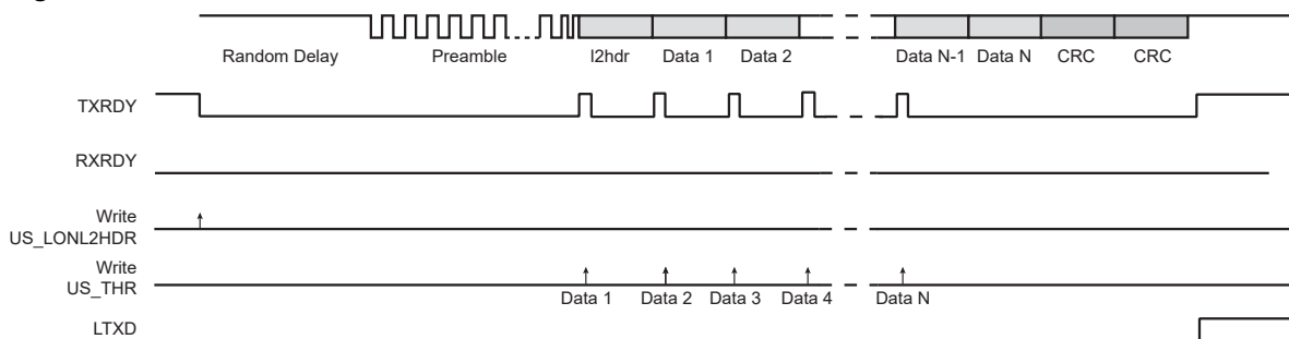
Figure 45-61. Tx Frame
