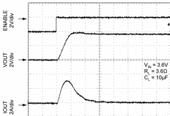
TIME 10µs/div
