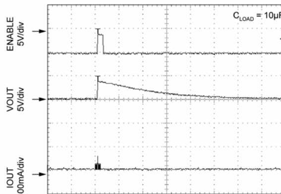
TIME 250µs/div
