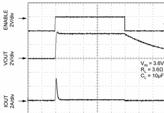
TIME 100µs/div
