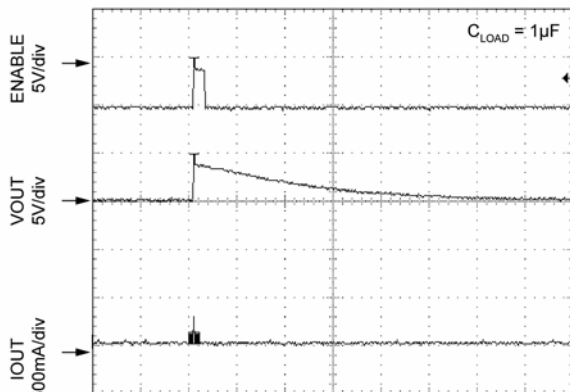
TIME 250µs/div
