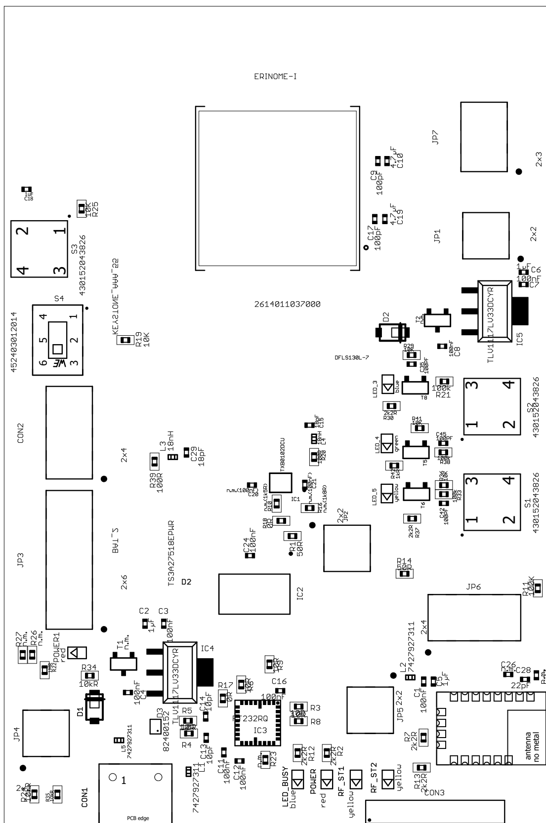
Figure 10: Assembly diagram
