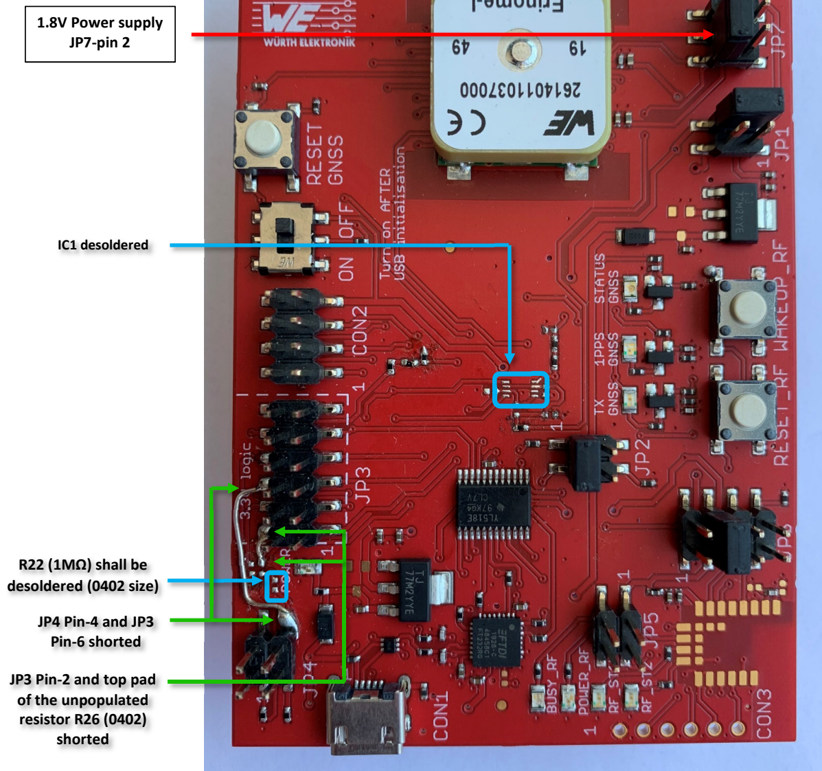
Figure 20: Modified evaluation board for SPI communication
