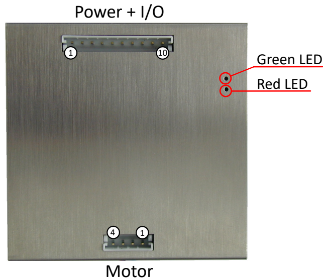
Figure 10: TMCM-1276 LED colors and loacation
