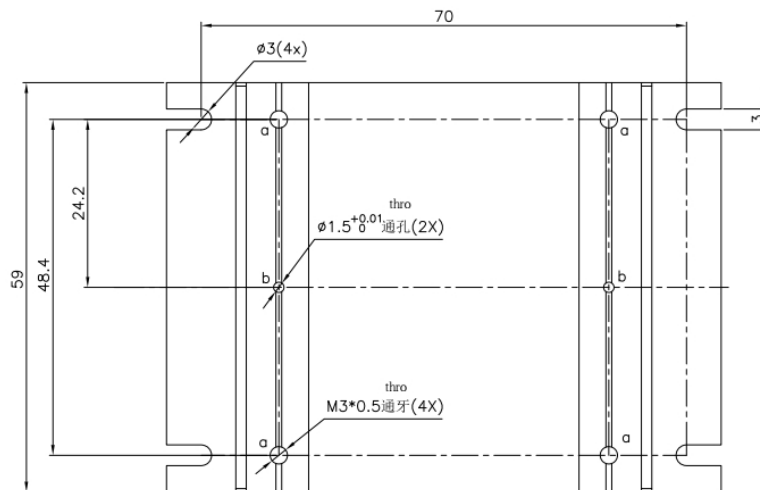
Figure 7: TMC-1276 housing base dimensions and screw hole positions
