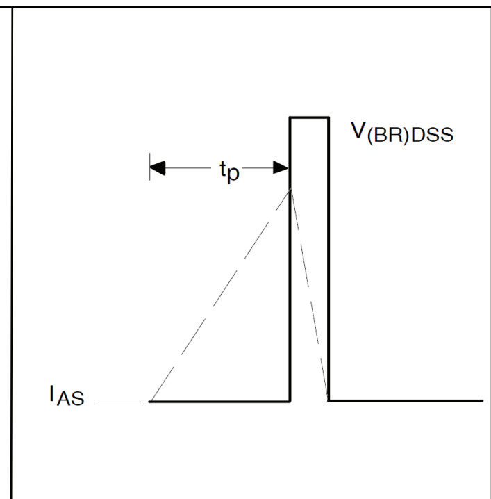
Figure 23b Unclamped Inductive Waveforms
