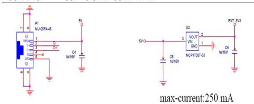
FIGURE A-8: USB TO UART CONVERTER
