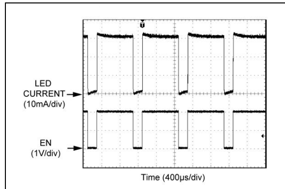
FIGURE 2-11: PWM Signal at 80% Duty Cycle.
