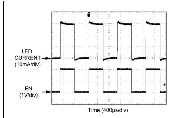
FIGURE 2-10: PWM Signal at 50% Duty Cycle.
