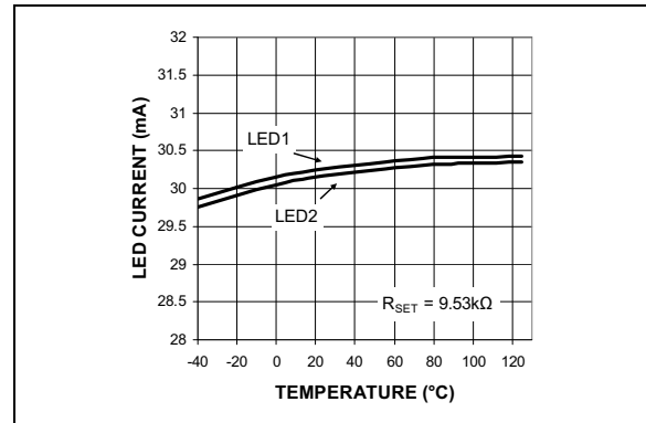
FIGURE 2-5: LED Current vs. Temperature.
