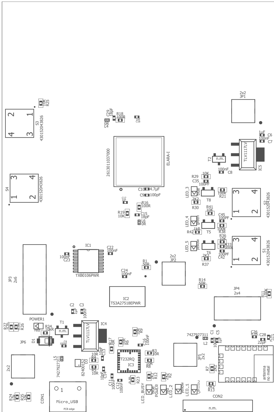
Figure 10: Assembly diagram
