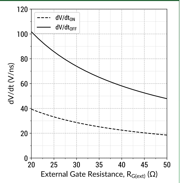
Figure 26: dV/dt v/s R_{G(ext)} ( V_{DD} = 1700V )
